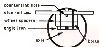
Figure 2 wheel details (side view)
