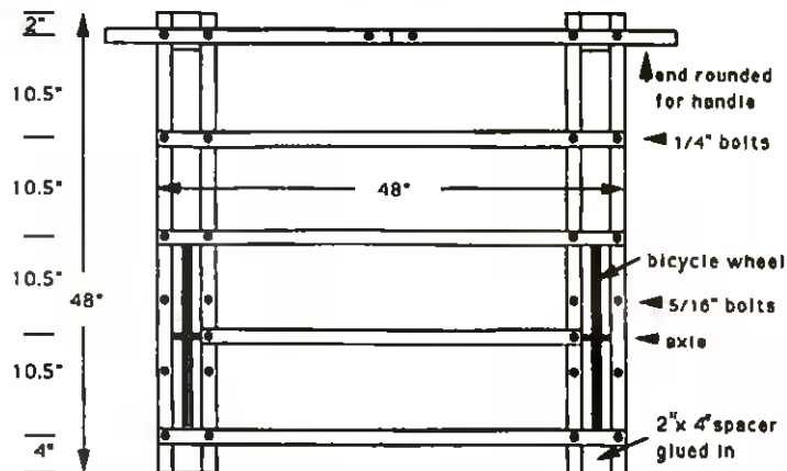
Figure 1 Assembly details (top view)
