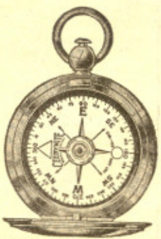
THE CEEBYNITE: —A luminous point, floating dial, hunter case model, made of white metal. The north and south points are treated with a permanently luminous radio-active compound, which makes them plainly visible at night. An automatic stop lifts the dial and needle off the centre point when the case is closed. Price $3.25
