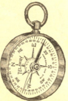
THE TELEWAY: —Has enamelled card dial, divided and figured. Special steel needle carefully magnetized and fitted with a jewelled centre. Brass case, finished in black bronze, diameter 1½ in. A heavy bevelled crystal serves as a cover, making the whole practically dust and water tight. Price 75c
