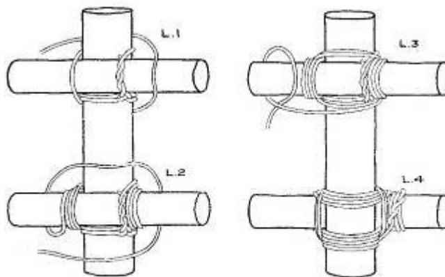
SQUARE LASHING
