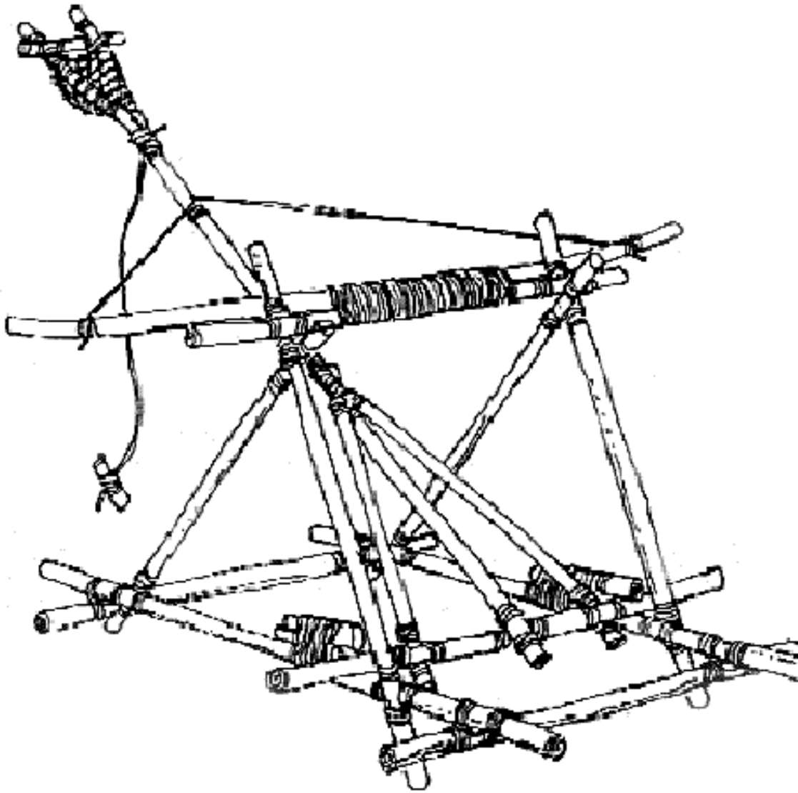
Troop 10 catapult
